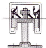
Typical Application of Trolley Assembly in UL1000 UtiStrut® Channel
