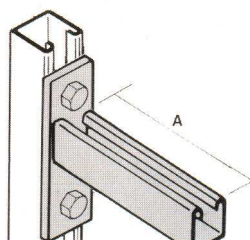
SS. Cantilever Arms Length A: 150mm 300mm 450mm 600mm 750mm
