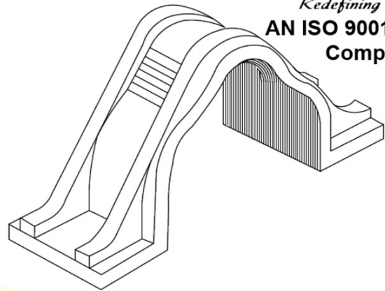
ISOMETRIC VIEW (3D)
