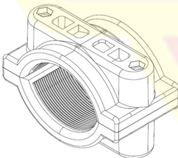
ISOMETRIC VIEW (3D)
